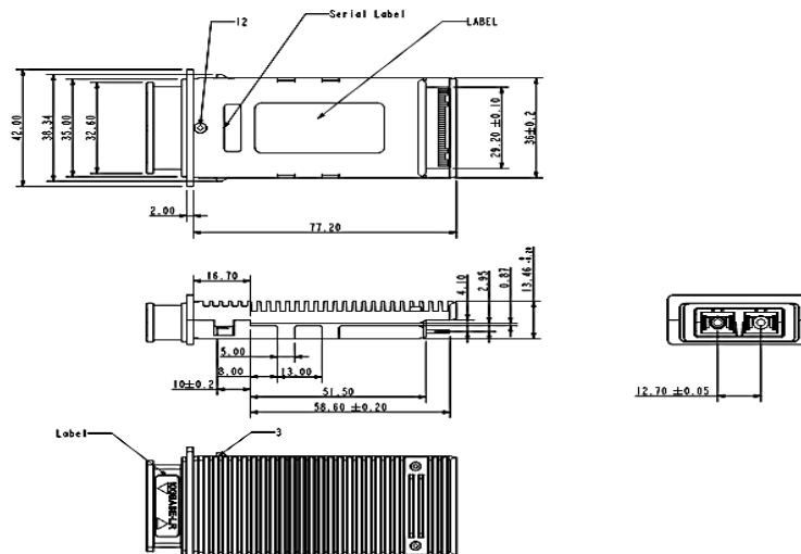
Figure 3: Mechanical Dimensions (Dimensions in mm)
